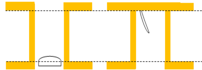
Figure 10-29: Examples of unacceptable voids
