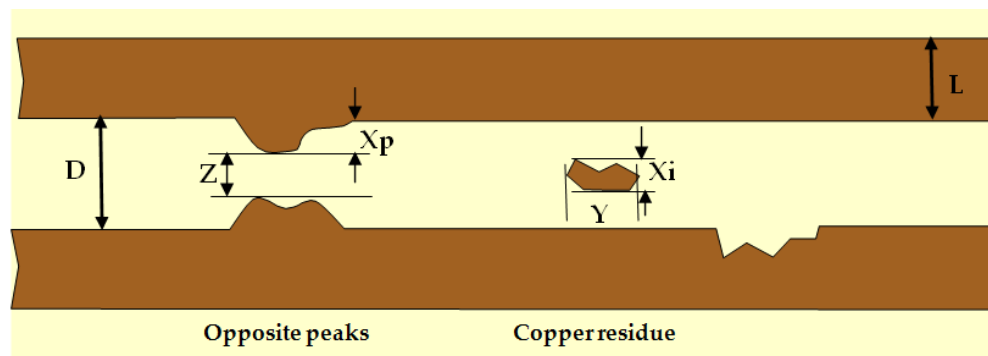
Figure 10-68: Conductor spacing
