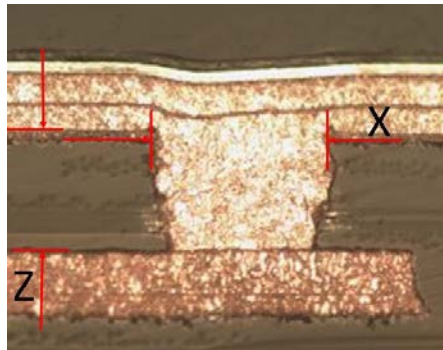
X=laser drilled diameter in layer 1 base copper, Z=distance from top of layer 1 base copper to top of capture pad copper
