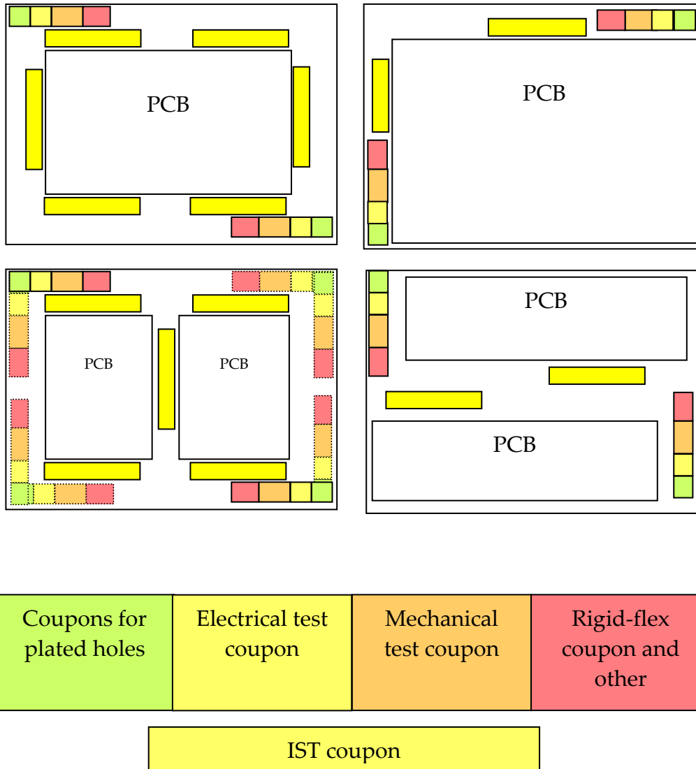
Figure 8-3: Example of placement of coupons and PCB in usable area of manufacturing panel
