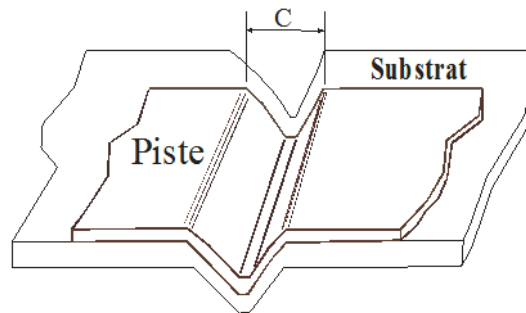
Figure 10-102: Copper wrinkle
