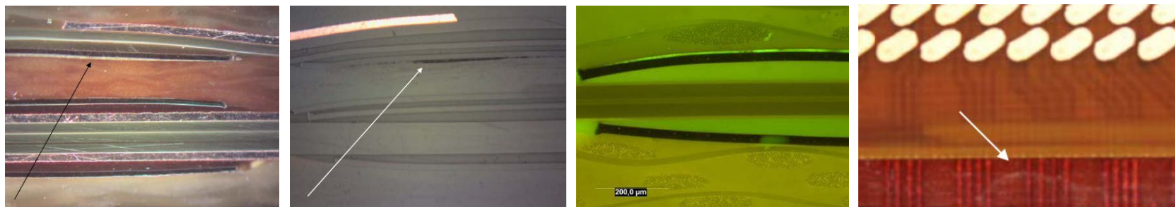
Figure 10-64: Delamination between coverlay and prepreg
