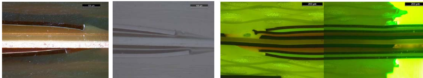
Figure 10-63: Acceptable adhesion between coverlay and prepreg
