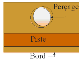
Figure 10-87: Misregistration of top and bottom coverlay
