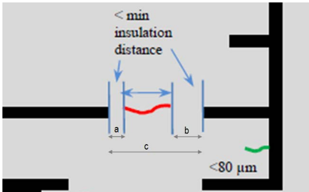
Figure 10-110: Calculation of remaining insulation distance
