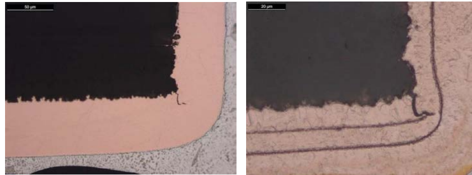
Figure 10-49: Example of C foil separation as-polished and after micro-etch
