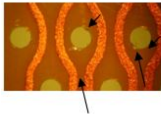
Figure 10-104: Burrs on holes
