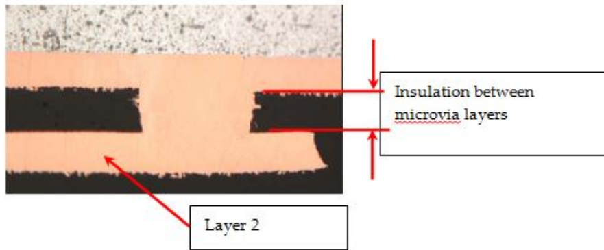
Figure 10-14: Microvia insulation
