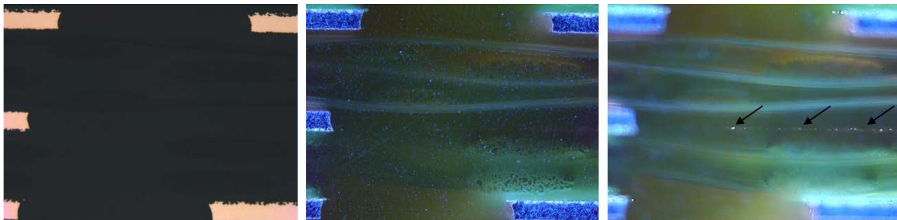
Figure 10-61: Example of dotted interface line observed in dark field out of focus (right), which is not visible in focus (middle) and in bright field (left)
