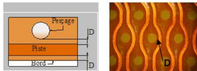
Figure 10-88: Misregistration of hole in coverlay to the conductor
