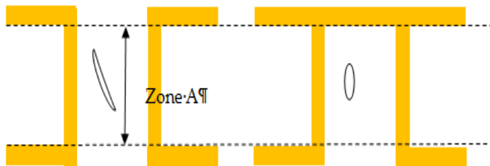
Figure 10-28: Examples of acceptable voids
