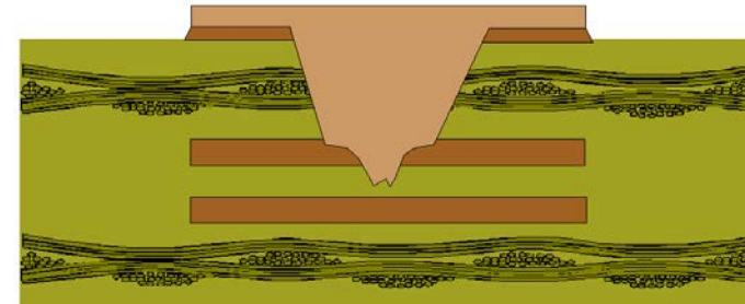
Figure 10-15: Penetration of capture pad for \mu\text{via} , not acceptable
