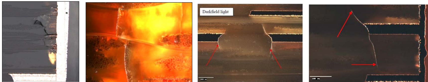
Figure 10-48: Examples of laminate cracks
