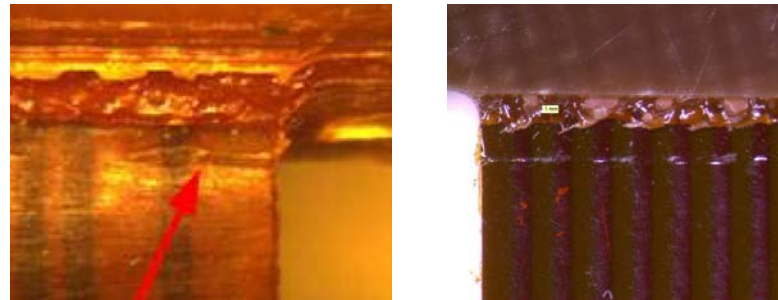
Figure 10-85: Examples of non-acceptable cut and blister, evident by a sharp indentation
