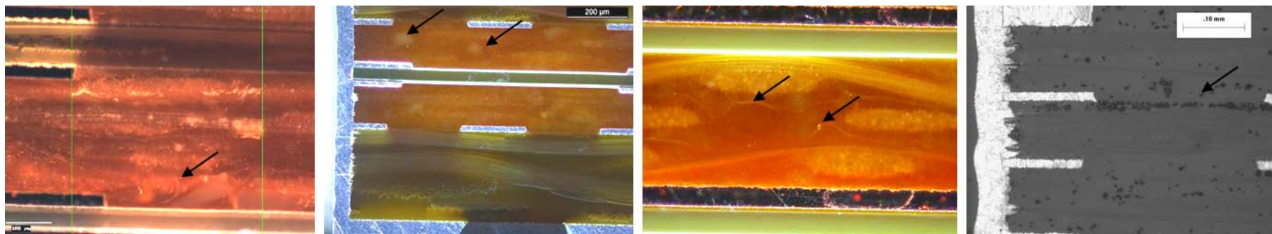
Figure 10-60: Examples of swirl (1 st and 2 nd image) and demarcation line (3rd). In the 2 nd picture the difference between no-flow prepreg (top) and laminate (bottom) is noticeable
