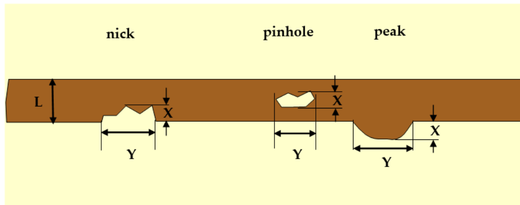
Figure 10-67: Conductor width
