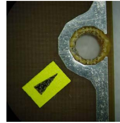
Figure 10-76: Haloing from non-plated hole to footprint for stiffener
