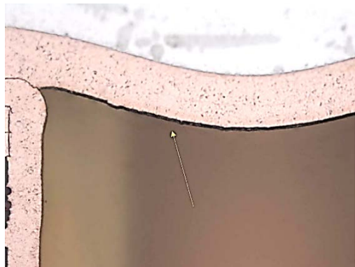
Figure 10-31: Example of acceptable thin line separation
