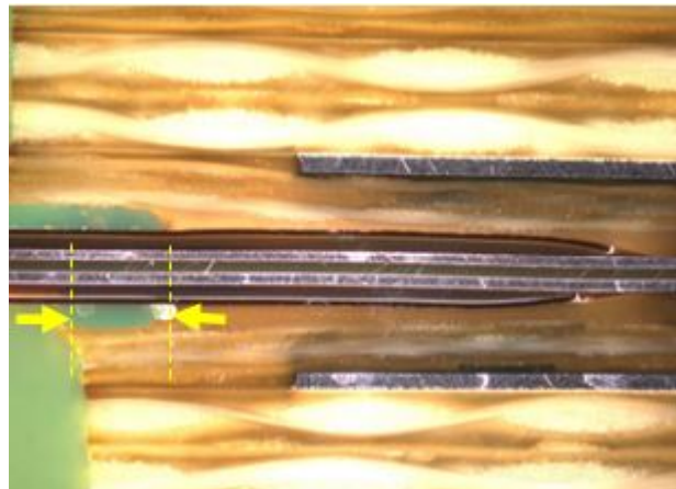
Figure 10-66: Example of adhesive filet recession into rigid section as observed in microsection
