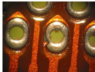
Figure 10-101: Pad diameter reduction due to local coverage by coverlay or resin squeeze out
