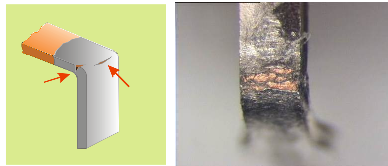
Figure 10-108: Unacceptable aspect of finger after bending
