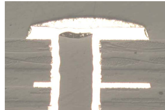
Figure 10-32: Example of non-acceptable bulging
