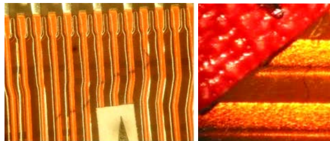
Figure 10-90: Examples of fibre contamination
