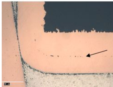
Figure 10-50: Example of interface line between plated copper layers on a non-etched microsection
