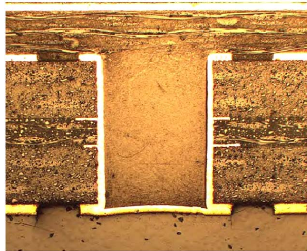
Figure 10-30: Examples of separation between hole wall and resin inside blind via
