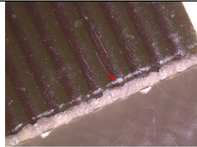
Figure 10-84: Example of an acceptable superficial scratch
