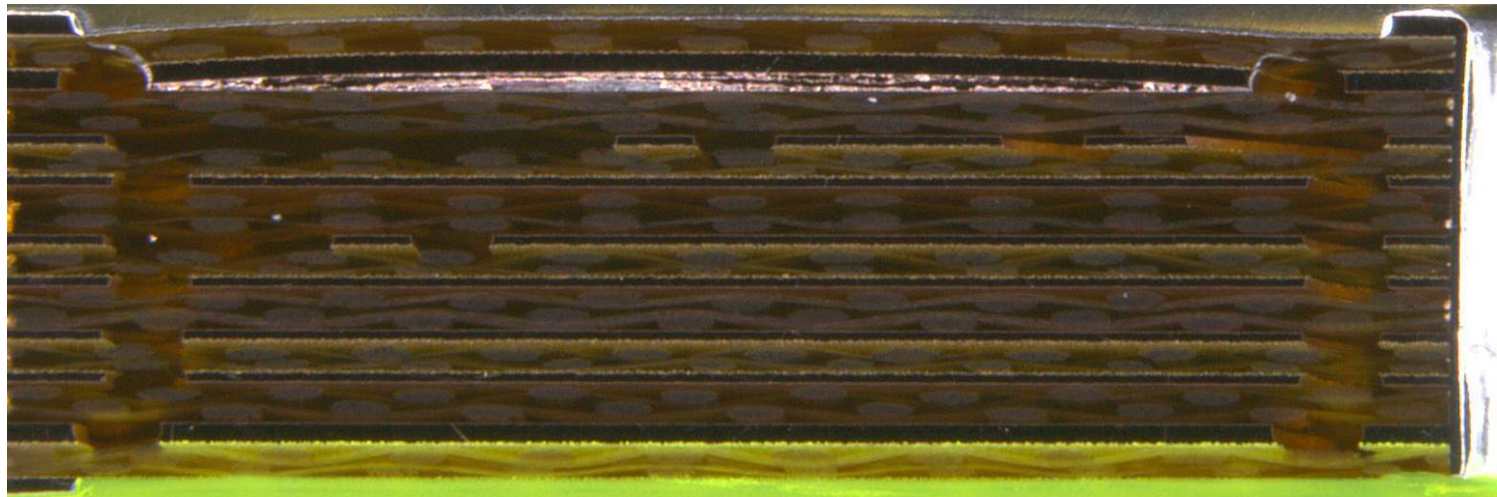
Figure 10-44: Example of delamination
