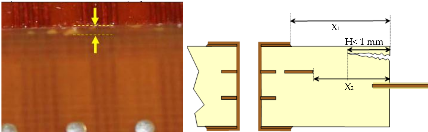
Figure 10-83: Example of acceptable incidental haloing \leq 1 mm into rigid section
