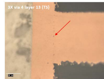
Figure 10-52: Examples of ICD
