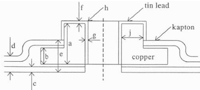
Figure 10-109: Cross-section of hole: Copper conductor shown
