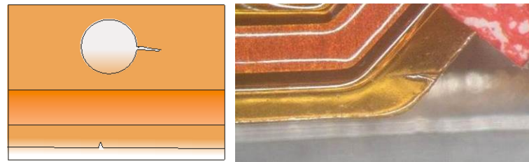
Figure 10-103: Tear in hole and edge of coverlay
