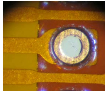
Figure 10-99: Example of adhesive in plated holes
