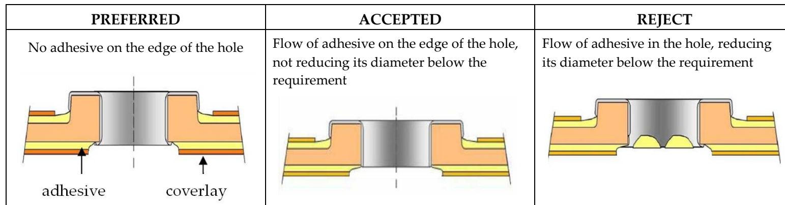
Figure 10-98: Adhesive in plated holes
