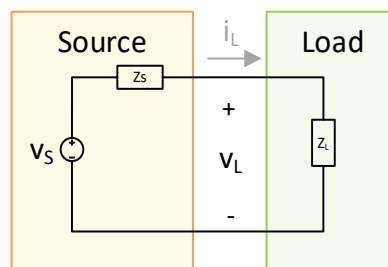
Figure 5-3: Thevenin equivalent model
