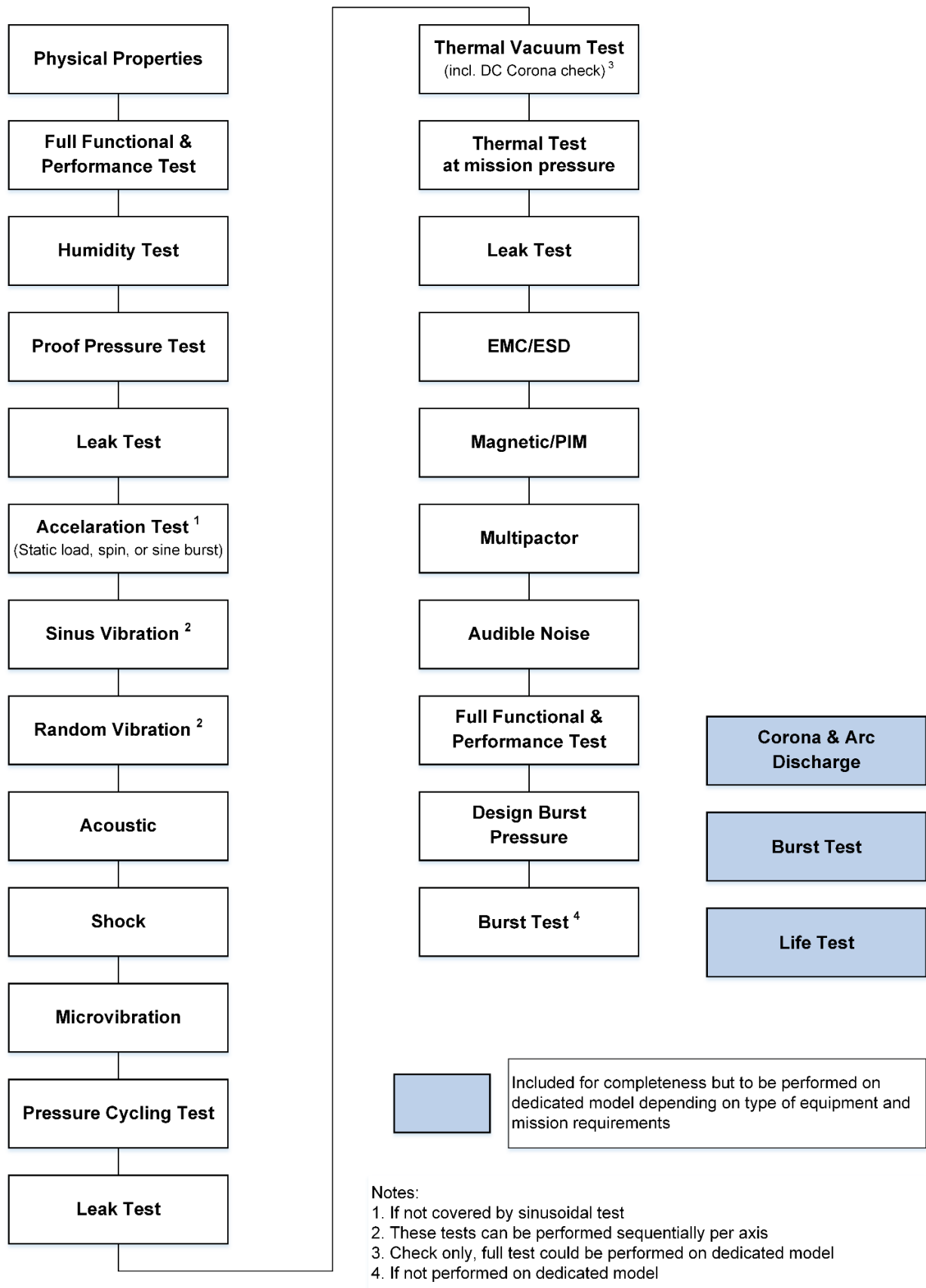
Figure 5-1: Space segment equipment sequence of tests
