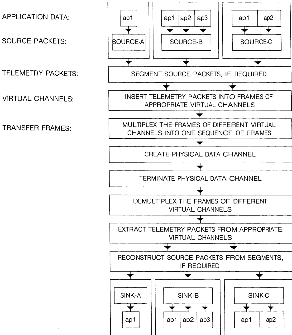
Figure 3.1 TELEMETRY DATA FLOW
