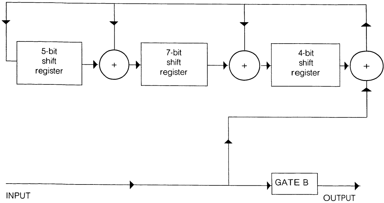
Figure C.1 ENCODER.
