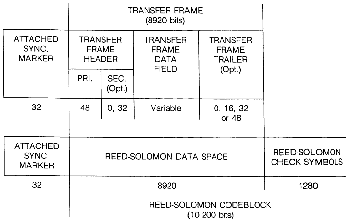
Figure 5.1 COMPOSITE TRANSFER FRAME/REED-SOLOMON CODEBLOCK FORMAT
