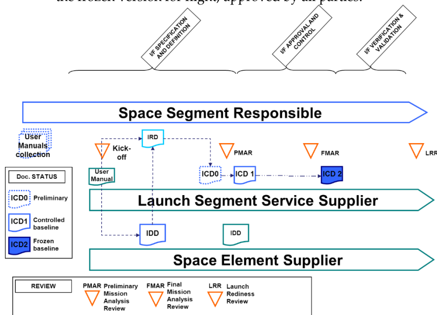
Figure 4-4: Typical space to launch segment interface life cycle
