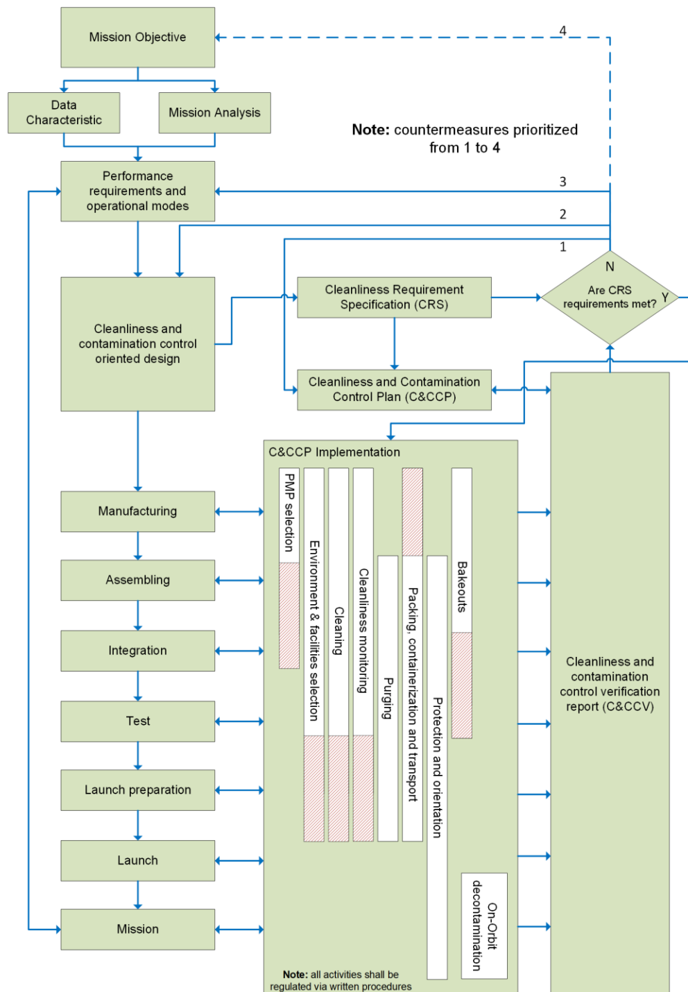
Figure D-1: Cleanliness and contamination control process overview
