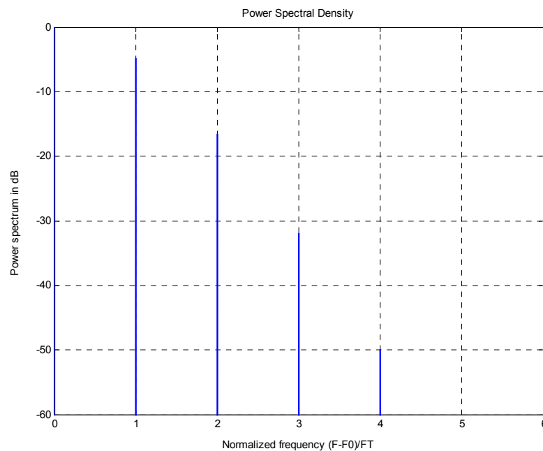
Figure 2: Ranging signal spectrum for code length = 2^0
