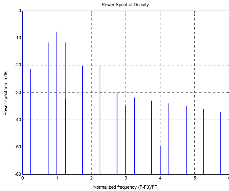
Figure 3: Ranging signal spectrum for code length = 2^2
