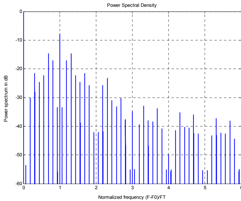
Figure 4: Ranging signal spectrum for code length = 2^4
