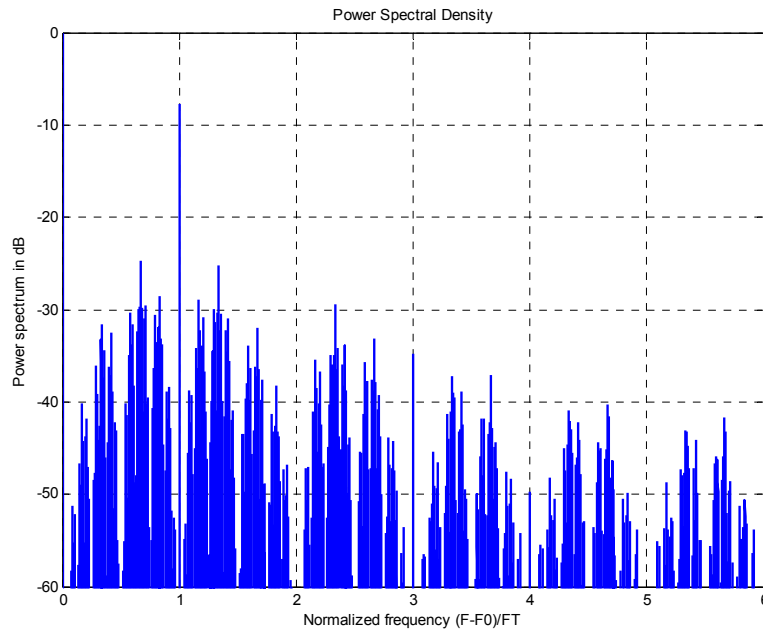
Figure 5: Ranging signal spectrum for code length = 2^{12}
