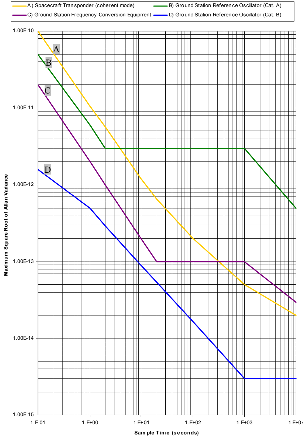
Figure 6: Carrier frequency stability requirements
