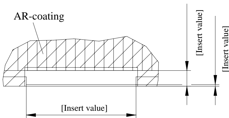
Figure C-3: BSC contact
